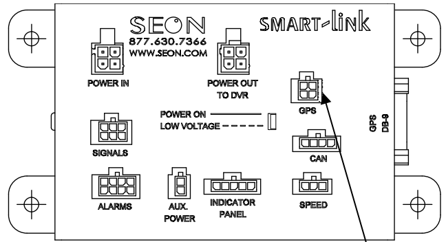
GPS receiver connector
